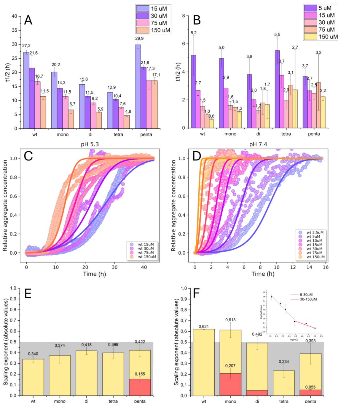
Figure 2. Macro- and microscopic analyses of aggregation kinetics of hIAPP variants at 37 °C at different pH values: 5.3 (A,C,E) and 7.4 (B,D,F). Half-time dependence of amyloid formation on the concentration of hIAPP variants at pH values of 5.3 (A) and 7.4 (B). Normalized ThT fluorescence intensity versus time for wt peptide at pH values of 5.3 (C) and 7.4 (D); 3–6 replicates were carried out. Absolute scaling exponent values versus hIAPP variants at a pH of 5.3 (E) and 7.4 (F); effect of high concentration depicted by red columns; an example of the slope change of the log–log plot of t_{1/2} versus m_0 for the mono variant (inset F).
