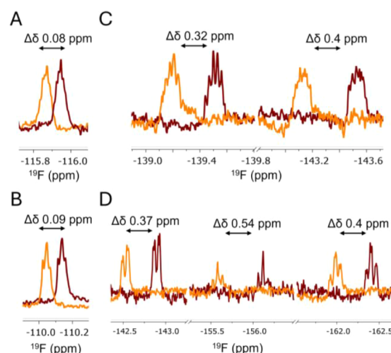
Figure 5. Conformational screening of hIAPP variants at the Phe23 region by ^{19}\text{F} NMR: red – pH 5.3 acetate buffer 30 mM (measured within the lag time), orange – Gdn \cdot HCl 6M; A – mono, B – di, C – tetra, D – penta.
